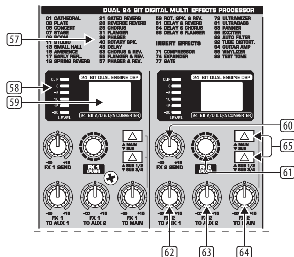
Fig. 2.25: The digital effects processor
