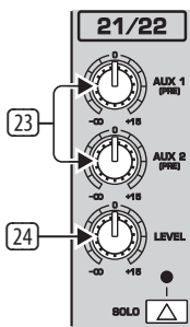
Fig. 2.8: Auxiliary stereo channels
