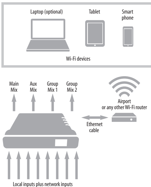
Figure 5-2: Using the 8D as a stand-alone mixer. This example demonstrates how you can control the mixer from several Wi-Fi devices.
