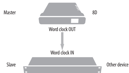
Figure 4-15: Slaving another digital audio device to the 8D via word clock. For the 8D clock source, choose any source besides word clock, as it is not advisable to chain word clock.
