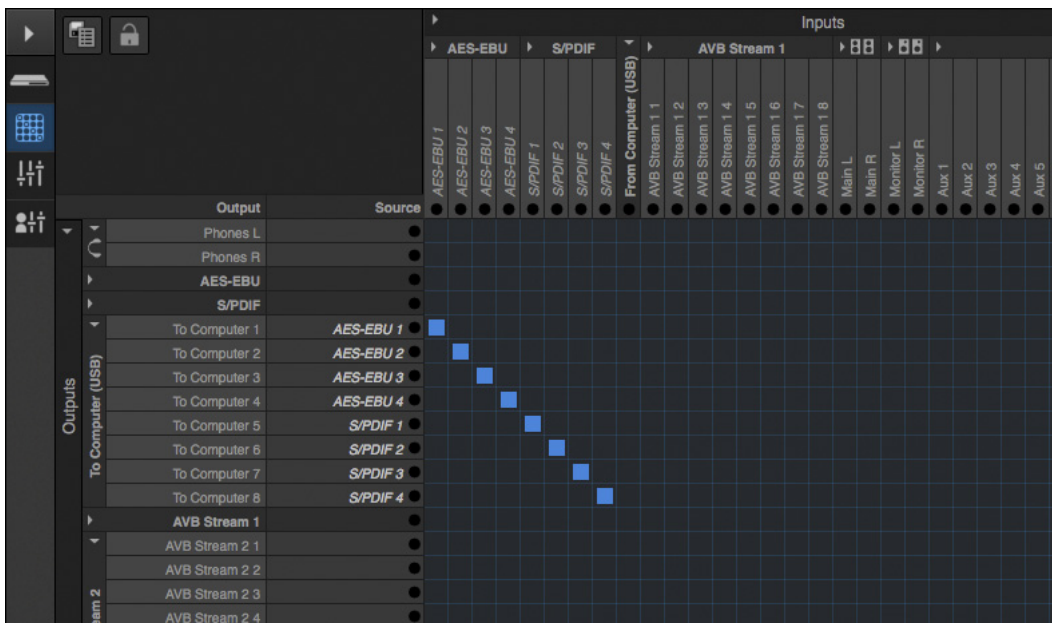
Figure 7-7: An example of routing physical inputs on the 8D to computer channels (for host audio software).
