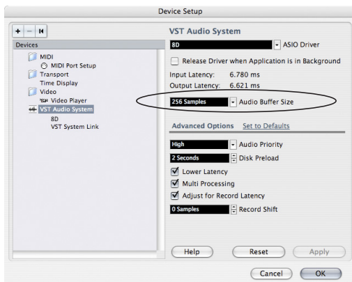
Figure 7-3: In Cubase or Nuendo, choose Devices menu > Device Setup. Select your interface (8D), then click the Control Panel button to access the window above and the Buffer Size setting.
