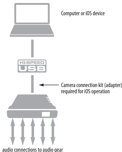
Figure 5-1: Using the 8D as an audio interface.
