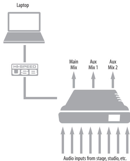
Figure 5-3: Using the 8D as an audio interface and mixer, simultaneously.
