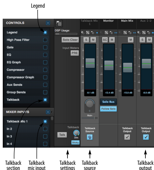
Figure 7-8: Mixer setup for the talkback mic.
