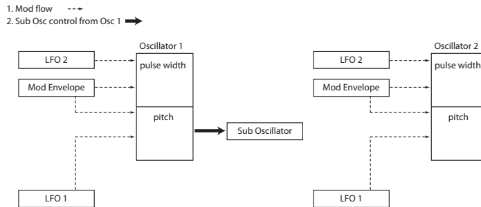
Oscillator modulation controls
